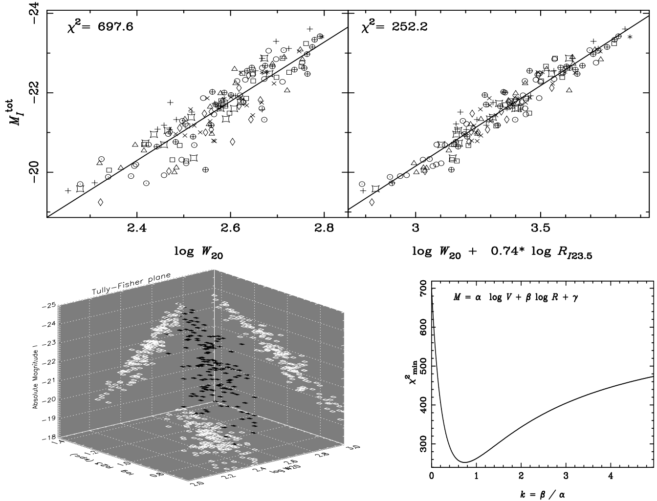
Fig. 1. Comparison of the Tully–Fisher relation (the left side) and the best fitting plane (the right side). Data of 160 galaxies were taken from Han (1992). The typical rms errors of the absolute magnitudes, together with the displacement from the uncertainties of W_{20} and R_{23.5} , were taken as 0.2 mag. Galaxies in different clusters were plotted by different symbols. The data distribution in 3-D space and the variation of fitting \chi^2 with k were also plotted.
